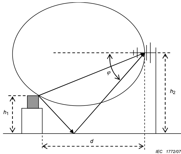
Figure 20 – Schematic of radiation from EUT reaching an LPDA antenna directly and via ground reflections on a 3 m site, showing the half beamwidth, \phi , at the reflected ray
